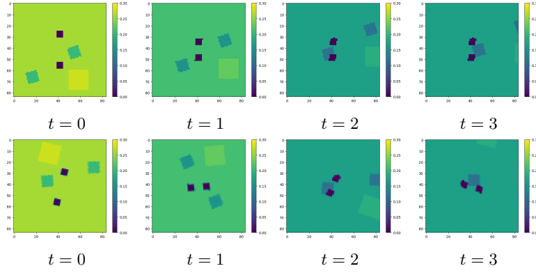
Figure 36: Examples of rotation data augmentation applied for transitions in an episode in Block-Pushing to augment the data for learning the representation: a different random rotation is applied independently for s, o, s', o' in each timestep in an episode.
