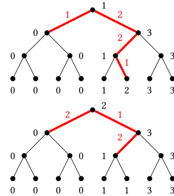
Figure 4: Refutation of the global median property on complete binary trees.
