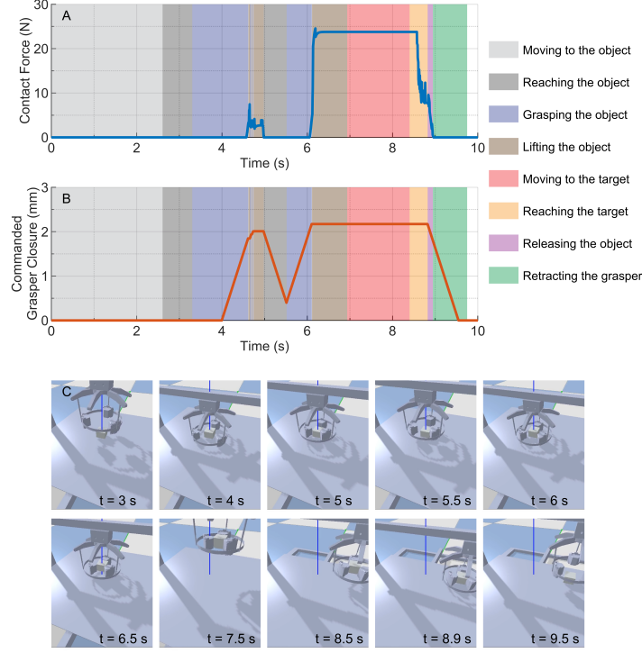
Fig. 4. The soft grasper controlled by the SNS network for pick-and-place manipulation in simulation. The object to pick up was a 500 g cube. Two attempts to grasp the object can be identified according to the contact force curve (A), the commanded grasper closure curve (B), and snapshots of the robot (C). The first attempt to grasp the object ( t=5 s) failed due to the low contact force. The grasper then attempted another grasp ( t=6 s). With the modulatory effect and increased force threshold, the grasper could successfully lift the object and move it to the target position. The colors of shades indicate the phases of the manipulation.
