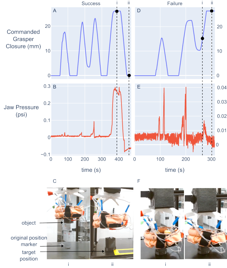
Fig. 7. Comparison of commanded grasper closure and jaw pressure for a successful (left column) and unsuccessful (right column) pick-and-place trial with the SNS modulation of force thresholds ( k = 29 ). While the commanded grasper closure shows an increase with subsequent attempts for both successful and unsuccessful grasp (A and D), the jaw pressure at the final attempt is much different (note the different y-axis scales of B and E). In the successful case, the grasper was able to deflate and successfully grasp the object (C, i) and deposit it at the target position (C, ii). In the failure case, the grasper did not fully deflate during the reaching-the-object phase of the reattempt, which caused the jaws to get stuck on top of the object (F, i). The commanded closure increased, but since the object was below the jaws, insufficient contact forces were generated to transition to the lifting-the-object phase (F, ii).
