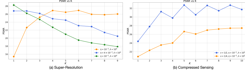
Figure 5: Ablation results of iteration number K on different tasks. For super-resolution and the other three tasks, K = 1 is sufficient to achieve the best performance with the optimal step size \eta and guidance weight \lambda . However, for compressed sensing, it is necessary to increase K to obtain the best performance. We hypothesize that this is due to the increased complexity of the compressed sensing operator, which requires more iteration steps to ensure the correct optimization direction.
