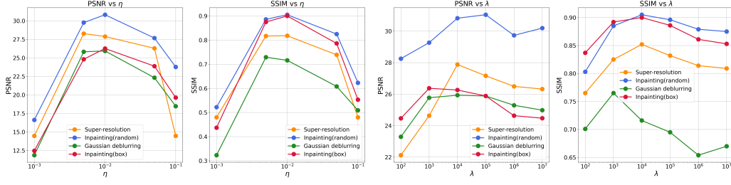
Figure 4: Ablation results of step size \eta and guidance weight \lambda . The choice of hyperparameters for our algorithm is fairly consistent across all tasks. We choose \eta = 10^{-2} for all experiments on CelebA-HQ. For \lambda , we choose \lambda = 10^3 for Gaussian deblurring and \lambda = 10^4 for the other tasks.
