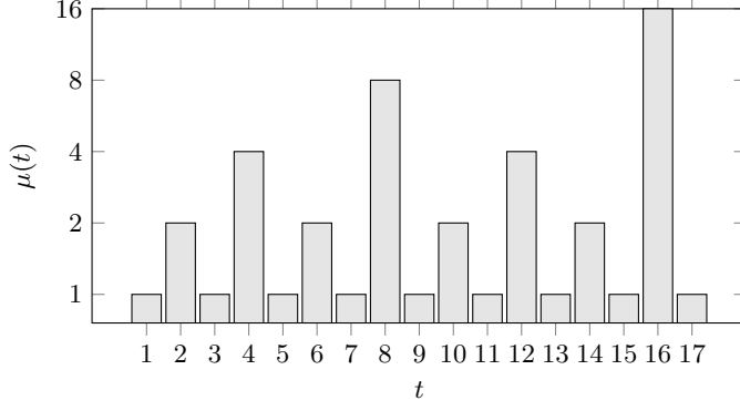
Figure 4: The capacities \mu(t) as a function of t .
