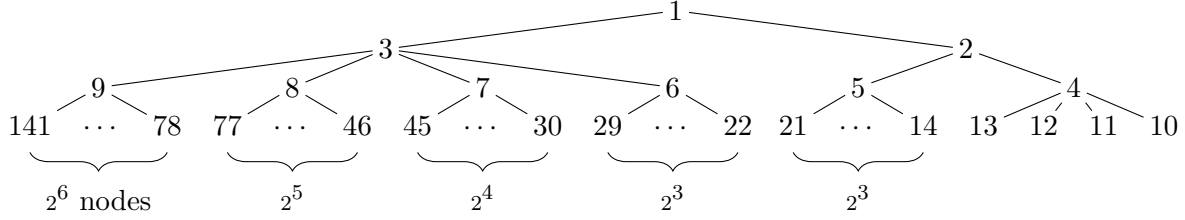
Figure 6: The top three levels of T_\infty . Each node i has 2^{i-p(i)} children, where p(i) is the parent of i (exc. p(1) = 0 ). The merge tree T_2^N (Figure 5) consists of these three levels, with each node i given weight 2^{N-p(i)} , so the nodes with weight 2^{N-i} are the 2^{i-p(i)} children of node i , and their total weight equals the weight of node i . Note that the label of a node in the merge tree is its weight, and the merge tree of Figure 5 is T_2^{18} .
