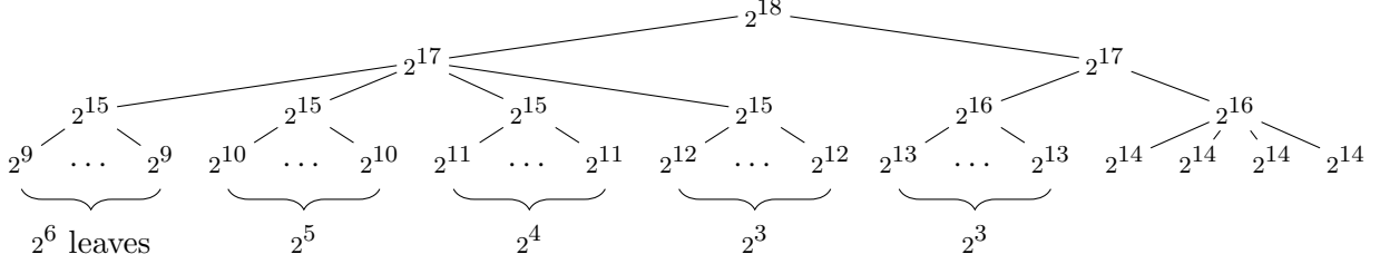
Figure 5: The “merge tree” for an execution of the Adaptive-Binary algorithm (Figure 3). The input sequence starts with m = 132 inserts I_1, I_2, \dots, I_{132} — one for each leaf, of weight equal to leaf’s label. It continues with 2^{16} - 132 empty inserts ( I_t = \emptyset ). At each time t = 2^9, 2^{10}, 2^{11}, \dots, 2^{17} (during the empty inserts) the algorithm merges all components of weight t to form a single new component, their parent. In this way, the algorithm builds a component for each node, with weight equal to the node’s label. At time t = 2^{17} the final component is built—the root, of weight 2^{18} , containing all items. The algorithm merges each item four times, so pays build cost 4 \times 2^{18} .
