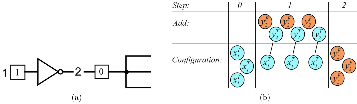
Figure 4: (a) A NOT gate with a fan-out of three. (b) Computing the NOT gate in Figure 4a in (2, 0) rules.
