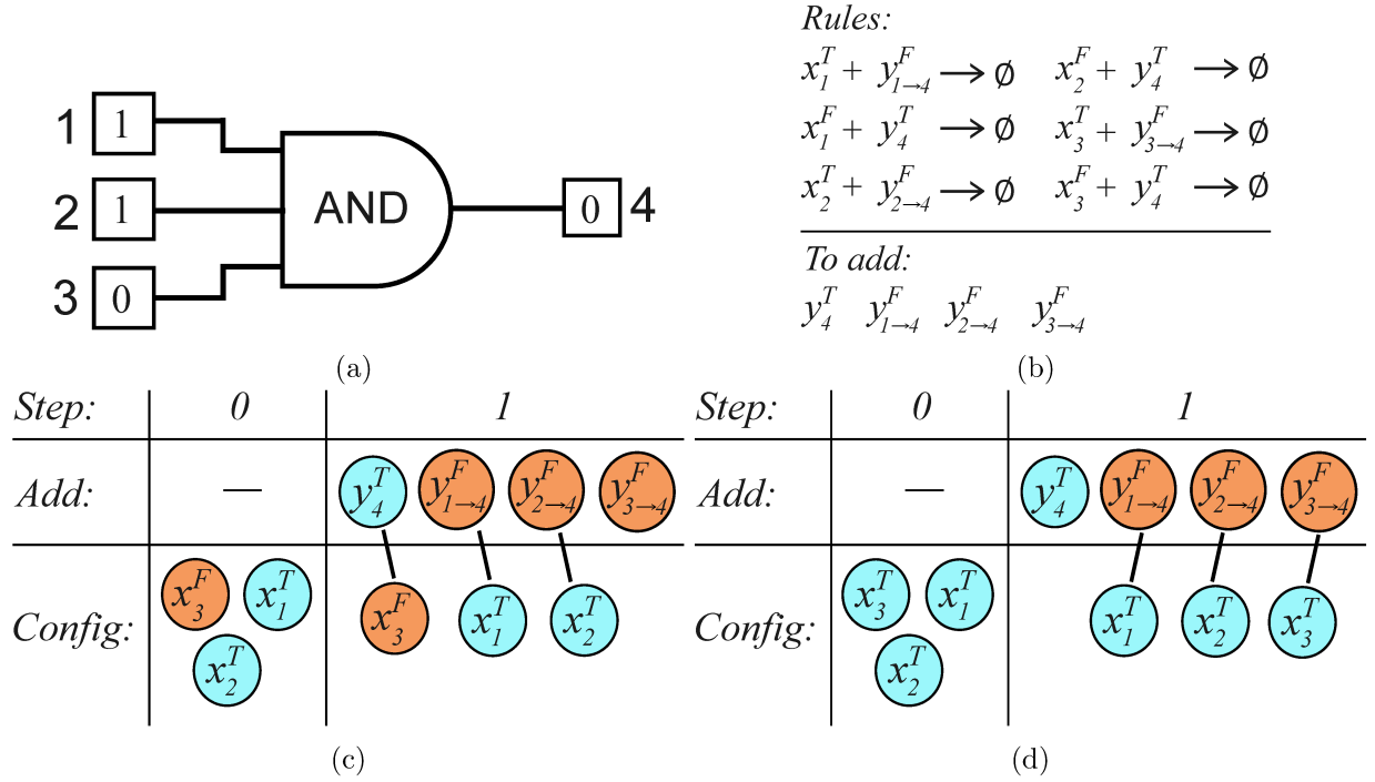
Figure 3: (a) A threshold formula consisting of a single three-input AND gate. (b) Reaction rules and added species for the step CRN that compute the formula in 3a. (c) The step CRN computing the formula in Figure 3a. The black lines connecting species represents a reaction applied to them. (d) The step CRN computing the circuit in Figure 3a, but with three true inputs.
