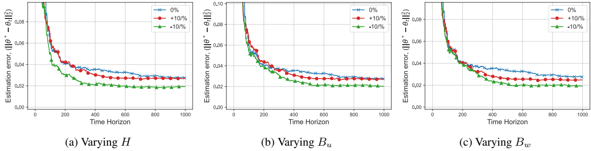
Figure 14. Estimation Error ( \|\theta^* - \theta_t\|_2^2 ) of Example I for three different values (standard and \pm 10\% ) of each hyperparameter while keeping the other hyper parameters fixed. The standard values of H , B_u and B_w are 45, 22876 and 0.6, respectively.
