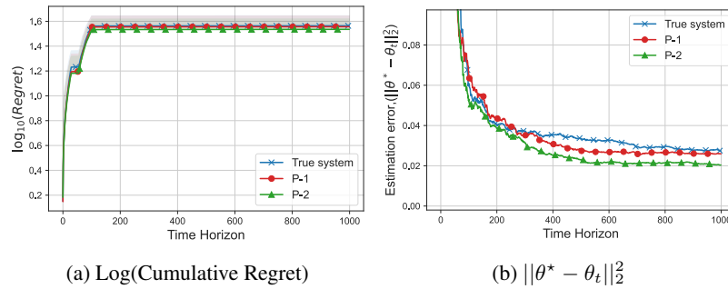
Figure 15. 15a and 15b are, respectively, the Log(Cumulative Regret) plot and the Estimation error plot of PIECE algorithm for the true system of Example I and two perturbed versions of the same system.
