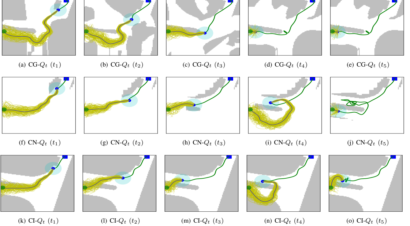
Fig. 3. Illustration of a grid environment with the starting point (blue square), robot's current position (blue circle), and the sensor field of view (cyan circle). The path traveled by the robot is shown in green, the yellow paths represent the default distribution with predicted mean path. (a) to (e) showcase the performance of the proposed method on the predicted map. (f) to (j) illustrate the performance of the CN- Q_t method on the observed map. (k) to (o) present the performance of the CI- Q_t method, which only considers sensor's field of view, the paths are overlaid on the ground truth map. All snapshots were captured simultaneously from the starting point to facilitate direct comparison.
