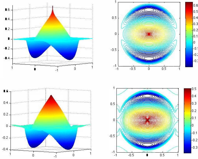
FIGURE 4.1. Solution of Bourgain-Brezis problem with 2D data in (4.11). Helmholtz solution, \mathbf{u}_{\text{Hel}} (top), vs. two-step solution, \mathbf{u}_{\text{2step}} (bottom).
