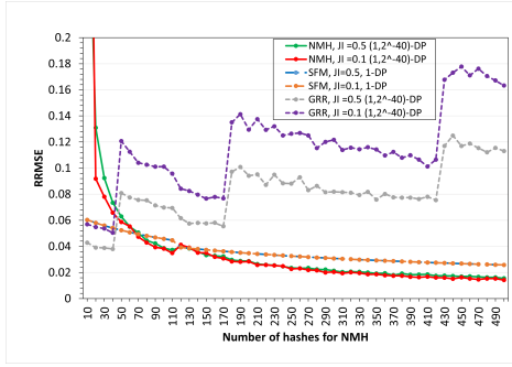
Figure 9: Accuracy: NMH, SFM, GRR.
