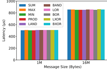
(a) Reduction Operations
