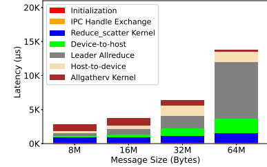
(c) Inter-node Multi-leader 2-level Designs
