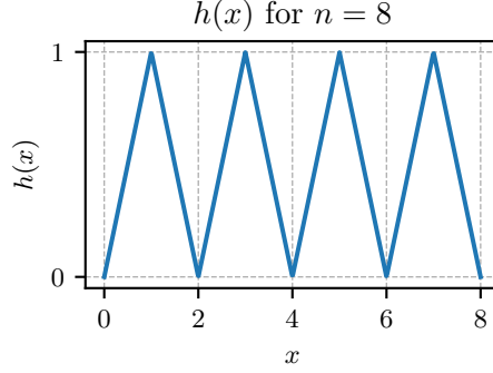
Figure 2: Sample form of function h(x) used in constructing g_{S,b}(\mathbf{A}) as a GNN. For the construction, we will have x = \sum_{i \in S} [\mathbf{c}_\mathbf{A}]_i .
