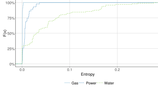
Fig. 4. CDF of packet size entropy
