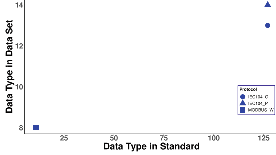
Fig. 6. Data Types.
