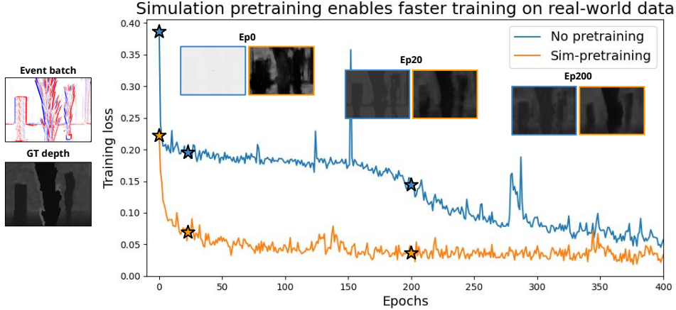
Figure S5: Simulation pre-trained (orange) events-to-depth models train faster on real data than non-pre-trained models (blue). Figure inserts contain evaluation examples of the predicted depth at epochs 0, 20, and 200 of training both models on real indoor data. Input event batch and ground truth depth are on the left of the plot.
