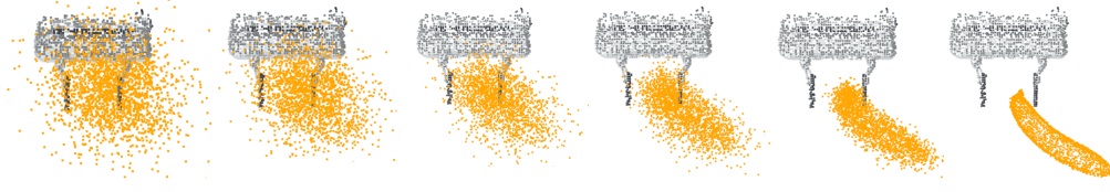
Figure 3. Trajectory of the pick generation process (“grasp the banana by the crown”). Unlike the place generation, our pick generation is conditioned on the canonicalized gripper point cloud. The generated point cloud at each timestep is colored in orange.
