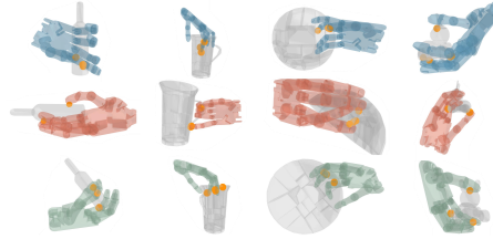
Fig. 5: Visualization of Contact Anchor . The yellow points are the generated contact anchors. Zoom in for a better view.
