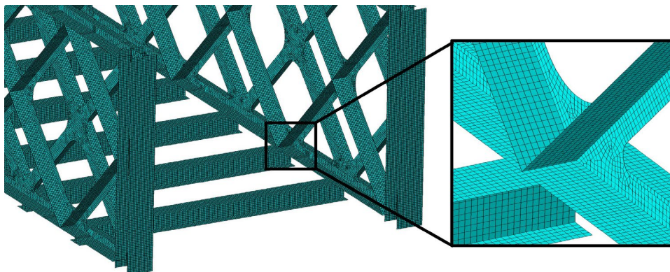
Figure 5: Finite element numerical model.
