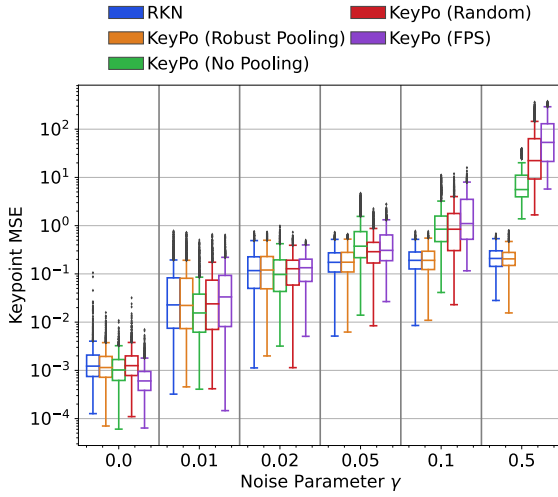
Fig. 6: Mean squared error (MSE) in the keypoint detection as a function of the added noise variance \gamma .
