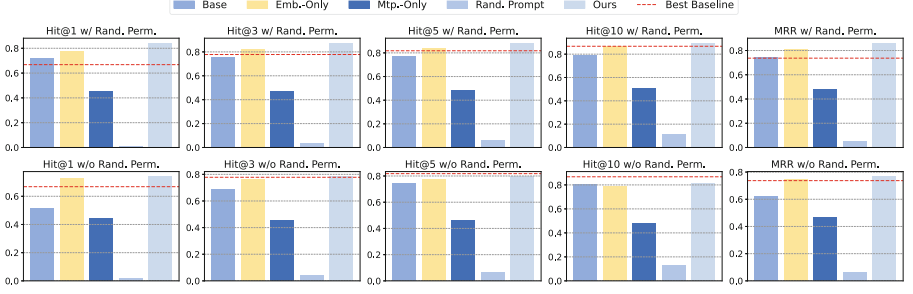
Fig. 4. Results of all component-differed variant models. The model variants in the first row randomly permute the input tokens, and the ones in the second row do not. The input tokens are constructed as indicated by the legend.
