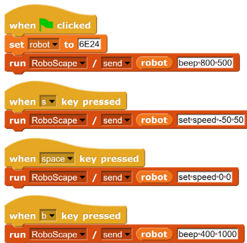
Fig. 12. Simple robot control program using keyboard events.
