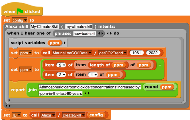
Fig. 24. Climate skill.
