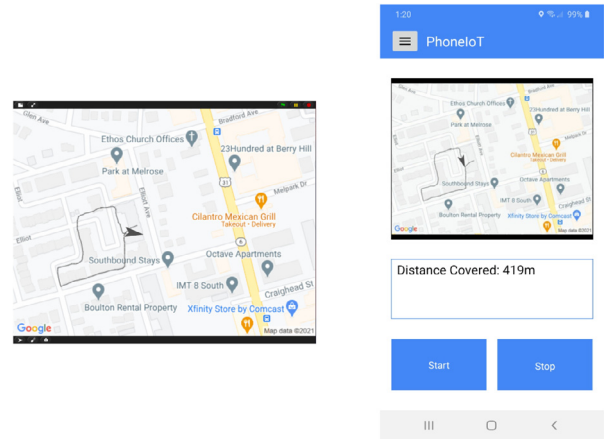
Fig. 23. NetsBlox client stage (left) and phone display (right) of the exercise tracker app at slightly different moments.
