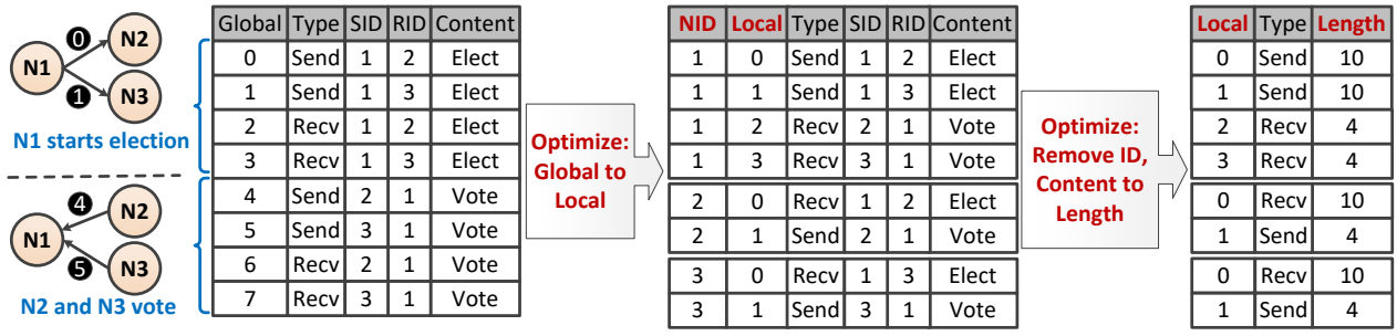
Fig. 8: Examples of DistFuzz's basic feedback encoding and various optimizations.
