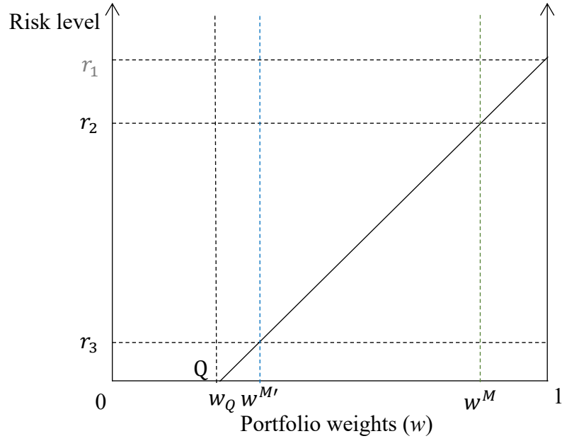
Figure 2. Consequences of failing to account for an upper limit constraint in MPT.
