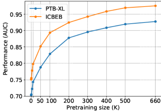
Figure 5: Performances of linear probing inference in arrhythmia diagnosis (AUC) on PTB-XL and ICBE data using the pretrained encoders with varying training samples.
