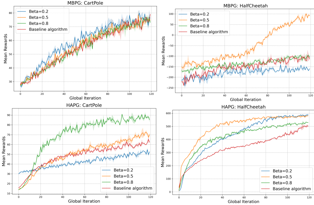
Figure 1. Mean rewards over global iterations for the CartPole and HalfCheetah tasks: (Top): FEDSVRPG-M; (Bottom): FEDHAPG-M.
