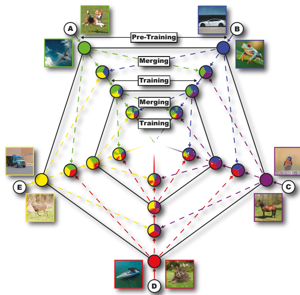
Figure 1. Illustration of DIMAT with ring topology for 5 agents. Agents, denoted by capital letters, undergo pre-training on two unique classes from CIFAR-10 each (solid lines). Subsequently, adjacent agents merge, forming tri-colored nodes (dashed lines). Updated agents then train on the original datasets (solid lines) with a slight increase in dataset colors. This merging and training cycle repeats for specified iterations until final fine-tuning.
