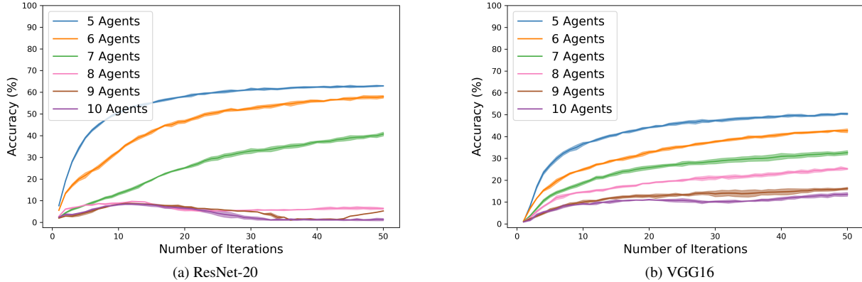
Figure 5. Scalability Analysis for DIMAT: Evaluating accuracy (mean \pm std) in fully connected topology with ResNet-20 (a) and VGG16 (b) on CIFAR-100 non-IID data across 5 to 10 agents.
