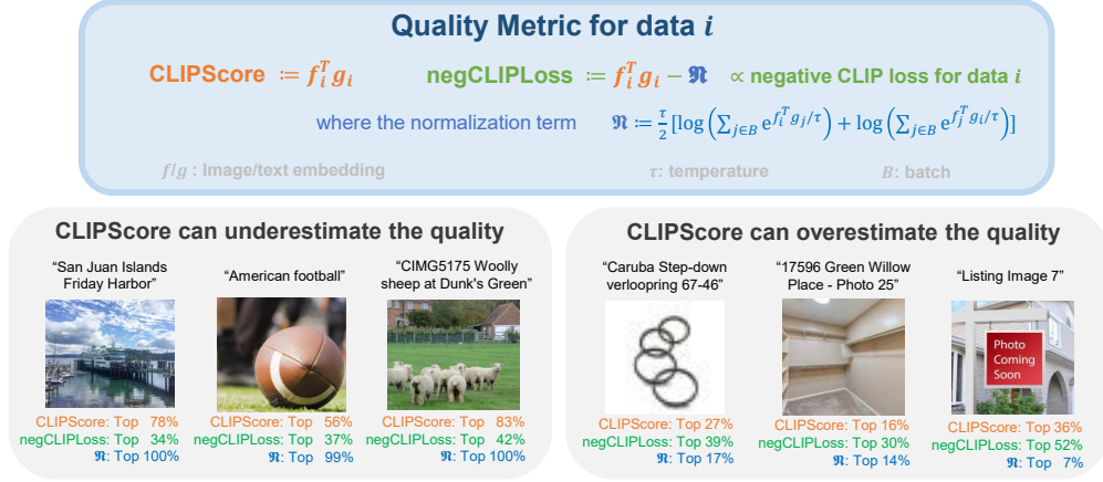
Figure 1: Illustration of negCLIPLoss. CLIPScore may underestimate (bottom left, where the data quality is high but CLIPScore is low) or overestimate (bottom right, where the data quality is low but CLIPScore is high) the quality of image-text pairs. However, this issue can be mitigated by simply subtracting a normalization term \mathcal{R} . negCLIPLoss employs the teacher model to calculate the negative CLIP loss on training data and serves as a more accurate metric. Here, “Top X%” denotes that the score represents the top X% high values within the entire dataset (i.e., the (100-X)% percentile among all the values). For example, “ \mathcal{R} : Top 100%” means this data has almost the smallest \mathcal{R} among the whole dataset, which represents that it contains highly specific elements in both images and texts.
