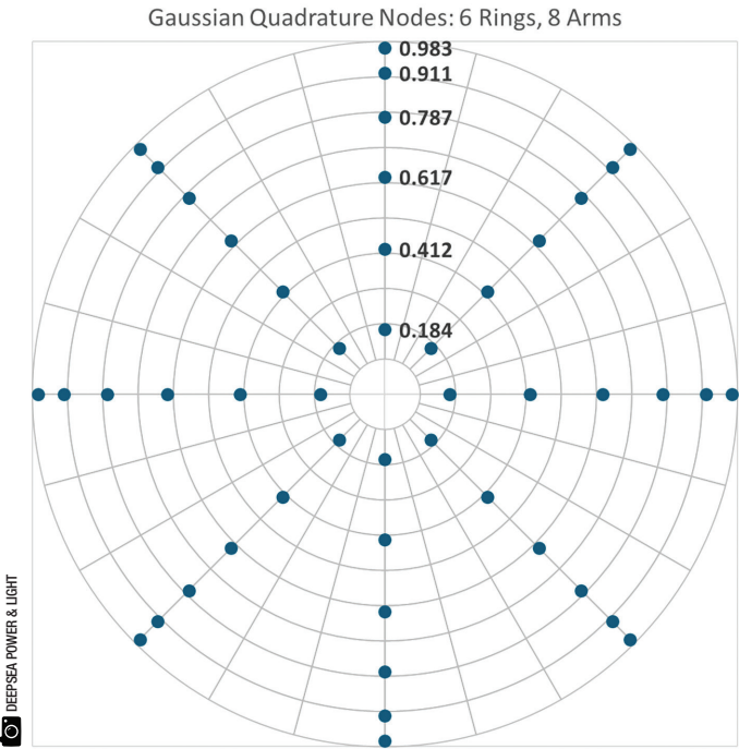
Figure 9 (left): Polar plot showing the distribution of node locations used by the Zemax merit function to evaluate the wavefront error of a simulated optical corrector during optimization. Rays of light at different wavelengths at these nodes are launched through the optics and the resulting projections produce a spot diagram. The Zemax merit function yields a weighted sum of the RMS radii of these projected spots as feedback to the optimizer to minimize the spot sizes across all of the nodes.
