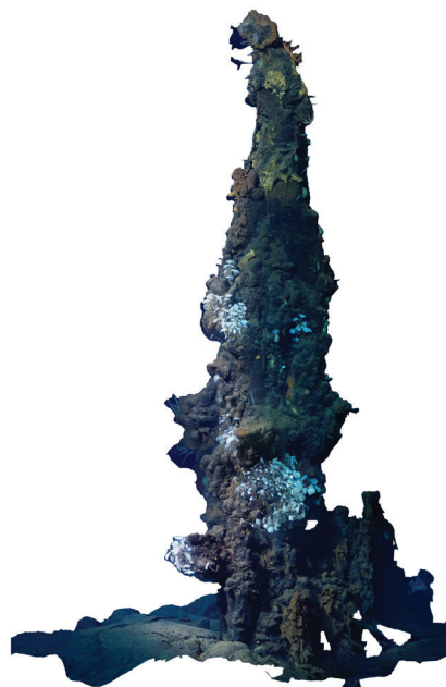
Figure 16: (Left) Sequence of digital screengrabs of an inactive hydrothermal vent colonized by a variety of sessile and mobile fauna, surrounded by lava likely erupted in ~2005-2006 at the East Pacific Rise near 9° 47'N west of the axis. Imagery is from 4K video acquired at 24 fps using a GoPro HERO4™ camera module in the 2nd generation MISO-OIS Super SeaCam housing. The camera was mounted on Alvin 's starboard arm during Dive 5236 in March 2024. (Right) The orthomosaic was assembled from a 3D reconstruction of 531 images extracted from the 4K video. The spire was imaged by moving the submersible up and down the structure in a scanning pattern. Agisoft Metashape ( https://www.agisoft.com/ ) was used to compute the 3D reconstruction and orthomosaic. No other post-processing has been performed on the imagery.
