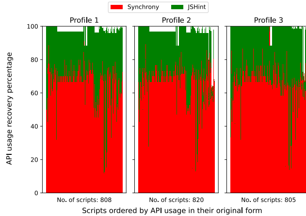
Fig. 5. Standard API recovery percentage between original and deobfuscated scripts by Synchrony compared between original and obfuscated code processed by JSHint versions for the obfuscation profiles (higher is better).
