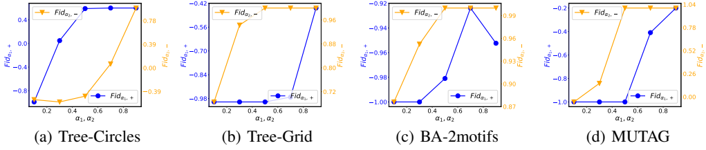
Figure 1: Parameter studies on the effects of \alpha_1 and \alpha_2 .
