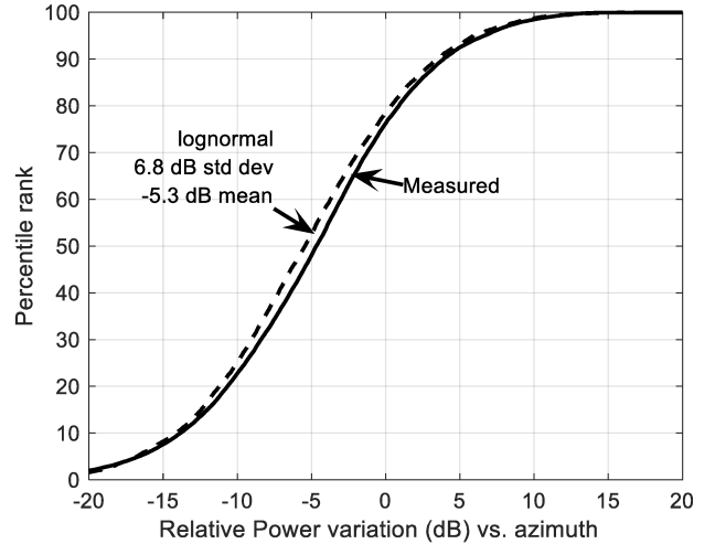
Fig. 3. Cumulative distribution of azimuthal variation of measured backscattered power ratio around local average.
