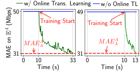
Figure 13: Online training cases (Left: C3 ; Right: C4 ).
