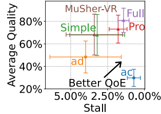
Figure 10: Quality vs. Stall of Habitue variants.
