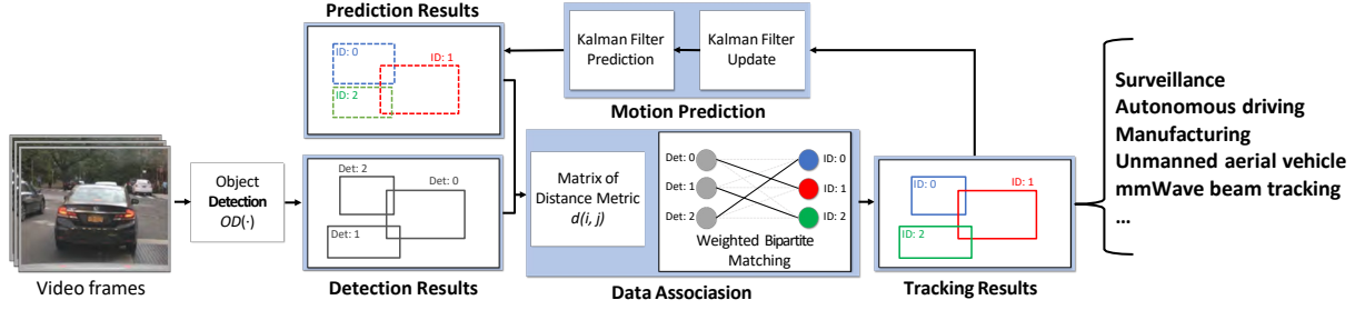
Figure 2: Illustration of tracking-by-detection pipeline in Multi-Object Tracking (MOT).
