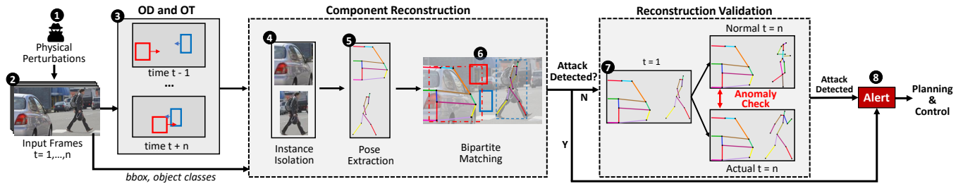
Figure 3: Illustration of VOGUES's stages.
