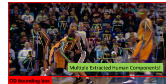
Figure 14: A common false positive case in sports tracking, where a crowd of people not in camera focus will be extracted as one bounding box by OD but have multiple components extracted. These cases are uncommon in the safety-critical domains of autonomous driving and surveillance due to the use of focus-free cameras.
