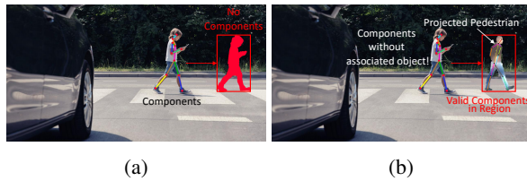
Figure 2: (a) Component consistency under tracker hijacking. (b) A naive attempt to evade component consistency by projecting a fake pedestrian into the hijacked tracker's position.
