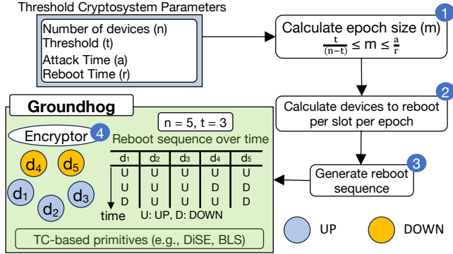
Figure 6. Overview of Groundhog . In Groundhog , we determine the reboot sequence using the given parameters t and n . We then calculate the size of an epoch using attack and reboot times. We use this epoch size and threshold t to find the number of devices we need to reboot per slot. Each device then uses this slot information and generated reboot sequence to find its next reboot time.
