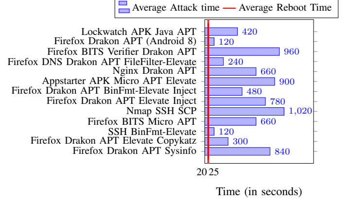
Figure 1. Average attack time for the attacks carried out by DARPA Transparent Computing (TC) program during Engagement #5 [5]. Note that the average reboot time for Amazon EC2 t3.xlarge instance (20.9 secs) and Raspberry Pi 4 Model B (25.2 secs) \ll the average attack time.
