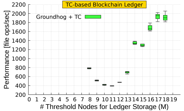
Figure 13. Performance of Groundhog in a TC-based Blockchain ledger application for various threshold number of nodes.
