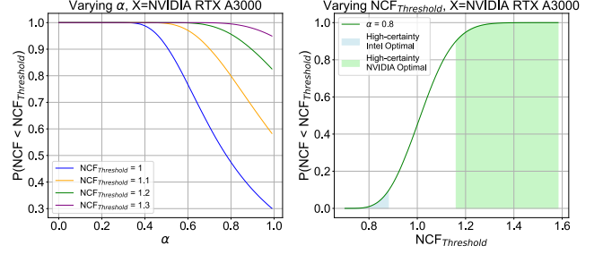
Figure 10: Probability of choosing correctly when choosing between the NVIDIA A3000 Mobile and the Intel A60M for various NCF_{Threshold} values (left) and for a fixed embodied-dominant regime where we show high-certainty decision making regions defined by the choice of NCF_{Threshold} (right).
