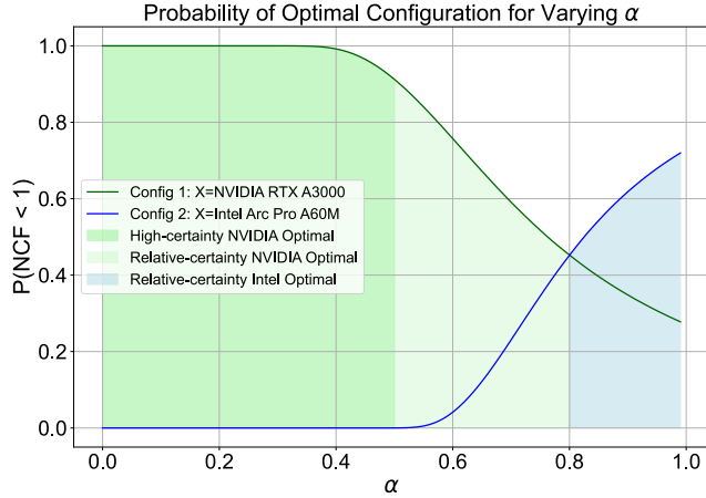
Figure 9: Probability of choosing correctly ( P(NCF < NCF_{Threshold}) ) when choosing between the NVIDIA A3000 Mobile and the Intel A60M across embodied and operational dominant regimes. We identify distinct regions where the optimal decision can either be made with high or relative certainty. The relative-certainty regions imply there is a significant probability that we will select a non-optimal GPU.
