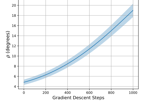
Figure 3: Angle \rho between \nabla_u L_{\text{srnk}} and \nabla_u L_{\text{uniformity}} across gradient descent steps. Fill represents std across three randomly initialized user matrices.
