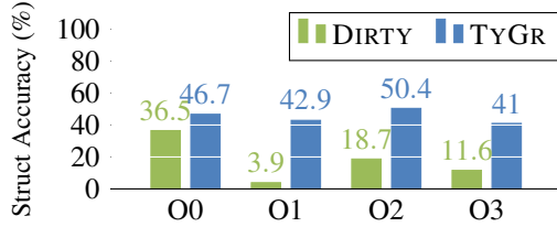
Figure 12: Accuracy of predicting struct types for TYGR and DIRTY on TYDA MIN x64 dataset.
