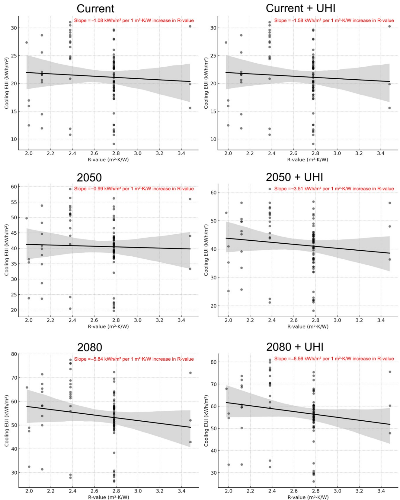
Figure 9. Cooling EUI sensitivity to R-value.
