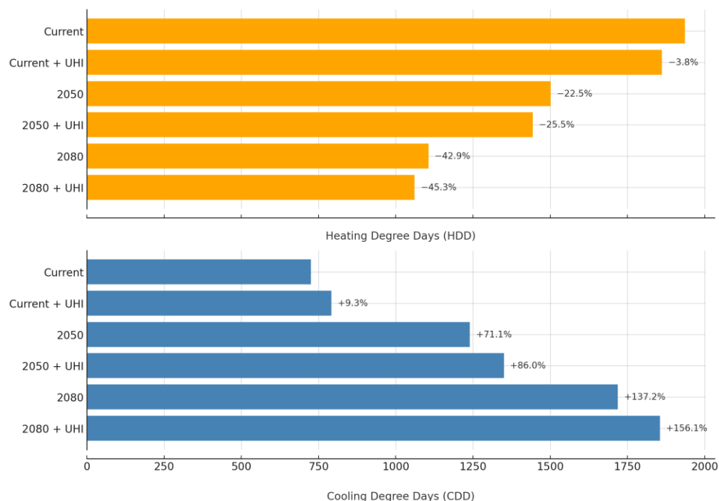
Figure 5. HDDs and CDDs across six weather scenarios.
