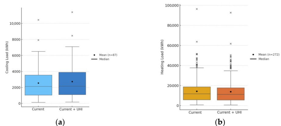
Figure 6. Cooling (a) and heating (b) loads under the current and UHI-influenced weather scenarios.
