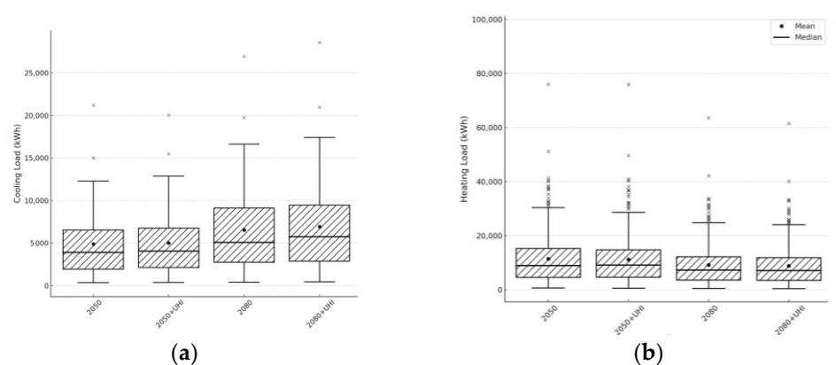
Figure 7. Cooling (a) and heating (b) load ranges across future weather and their UHI-induced scenarios.
