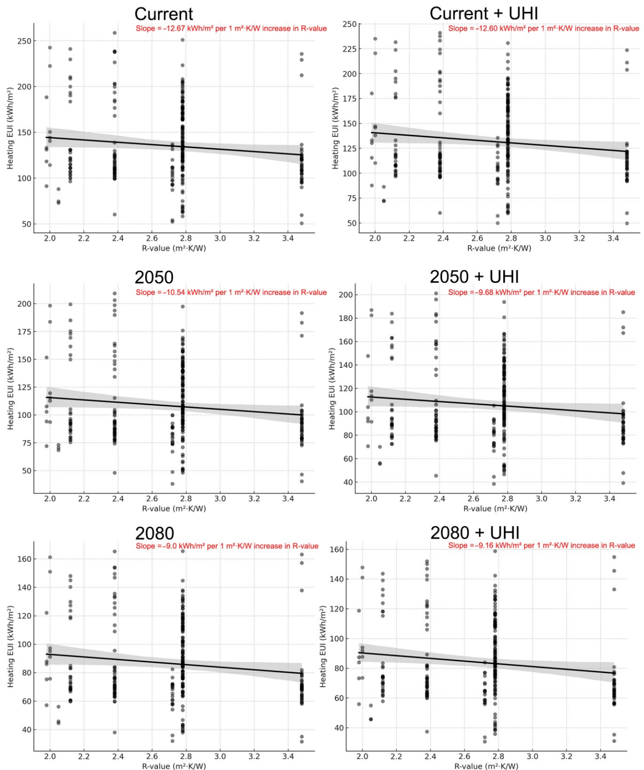
Figure 10. Heating EUI sensitivity to R-value.
