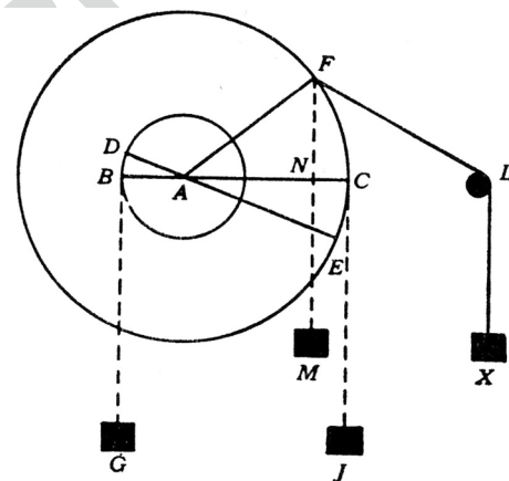
Fig. 8 Galileo's diagram for the Windlass, with J as a small weight that can raise a larger weight G (from Galilei 1960)
