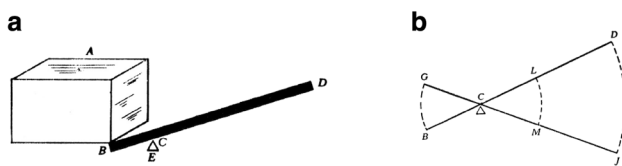
Fig. 5 a Galileo's Prybar, b Galileo's skeletal diagram for a Lever (from Galilei 1960)
