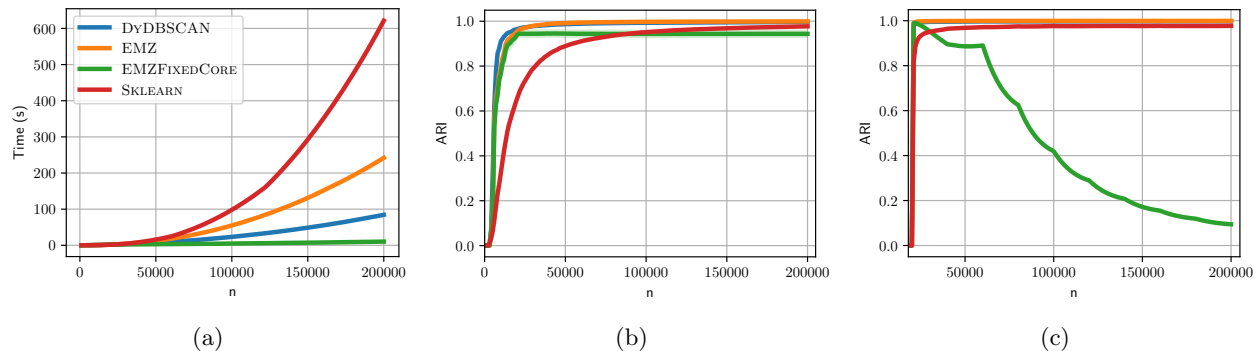
Figure 2: Comparison on the blobs dataset. (a) The running time of each algorithm. (b) The ARI for each algorithm when data points are added in a random order. (c) The ARI for each algorithm when data points are added cluster-by-cluster.
