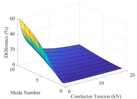
Fig. 12. Difference between the analytical beam model and analytical string model with tension.
