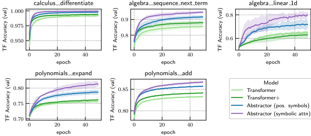
Figure 7: Training curves comparing an Abstractor-based architecture to a standard Transformer on mathematics problem-solving tasks.
