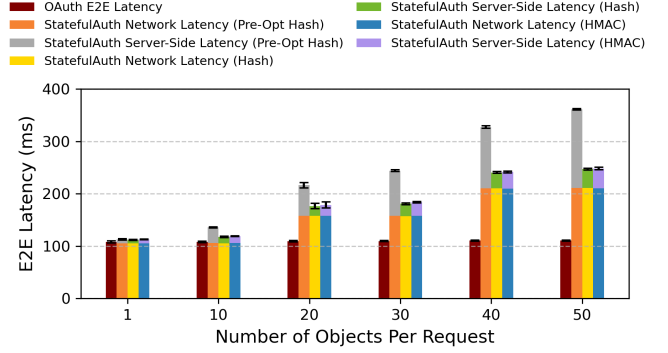
(a) End-to-end latency of OAuth and StatefulAuth (Hash- and HMAC-based integrity).
