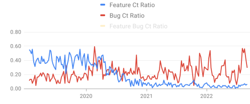
SWE Coding Time Feature-Bug Ratio by Week
