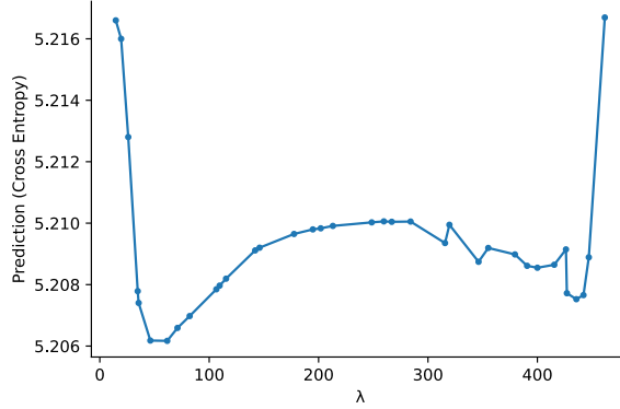
Figure 4: Cross entropy as function of \lambda across for symbolic sequence generated by HMMs.
