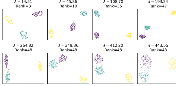
Figure 3: Learned representations for symbolic sequences generated from Hidden Markov Models (HMMs), recovered by solving Program (5) with varying nuclear constraints \lambda , visualized using UMAP projection.
