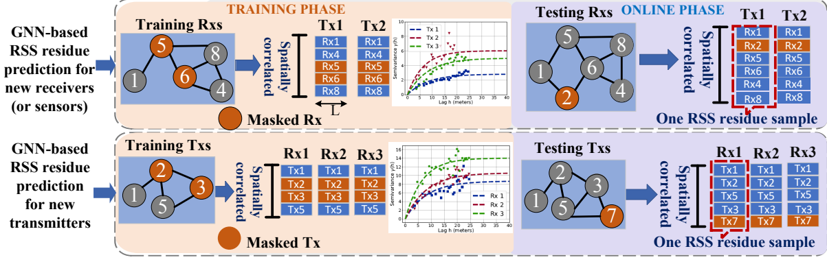
Fig. 3: Illustration of GNN training and inference.
