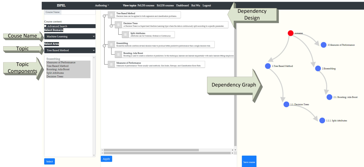
Figure 3: An instructor can choose topics (i.e., select area, see left top corner), select topic components, and design how to connect topic components (see middle column) with a book chapter and sub-chapter style to define the dependencies. When the “Apply” button is clicked, a dependency graph will be generated automatically.
