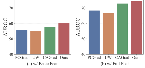
Figure 7: Performance of HTP-Star with different balancing method.
