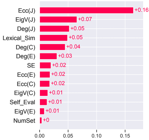
(c) Shapley Values: XGBRF
