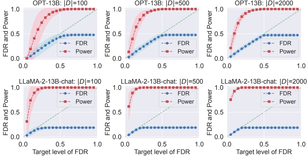
Figure 12: FDR/power plots for conformal alignment with CoQA dataset and XGBRF as the base classifier. Details are otherwise the same as Figure 3.
