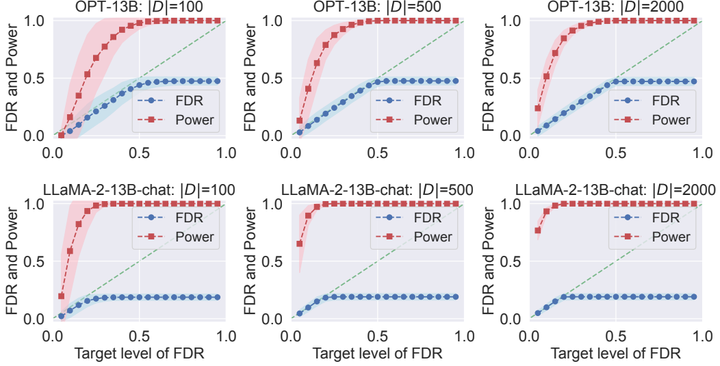
Figure 10: FDR/power plots for conformational alignment with CoQA dataset and logistic regression for training the alignment predictor. Details are otherwise the same as Figure 3.
