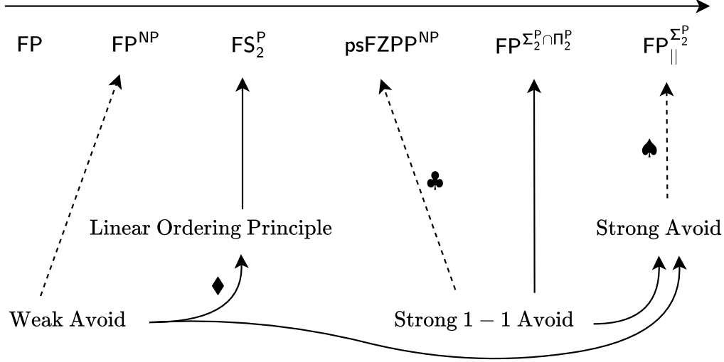
Figure 1: Inclusion diagram of relevant classes and search problems. Solid arrows represent the inclusion of the class at the base of the arrow into the class at its tip. Dotted arrows indicate non-inclusion of the base class into the tip class in the decision tree model. The main linear axis of classes along the top are all included from left to right, indicated by the long solid arrow above them. Our major results are the separations marked with ♠, ♣ and the inclusion marked with ♦. \text{TFU}\Sigma_2^P essentially corresponds to \text{FP}^{\Sigma_2^P \cap \Pi_2^P} , see Lemma 2.
