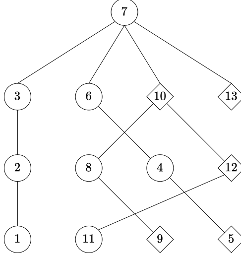
Figure 2: Example instance of Forest Termination with M = 4 and N = 3 , with virtual root added at the top. Blue nodes are circles and red nodes are diamonds. We have sorted each layer left to right so that blue nodes come first, and within each color class the nodes are ordered left to right lexicographically. The number on each node represents its position in the ordering \prec . The nodes numbered 1 and 4 are the termination points of this instance.
